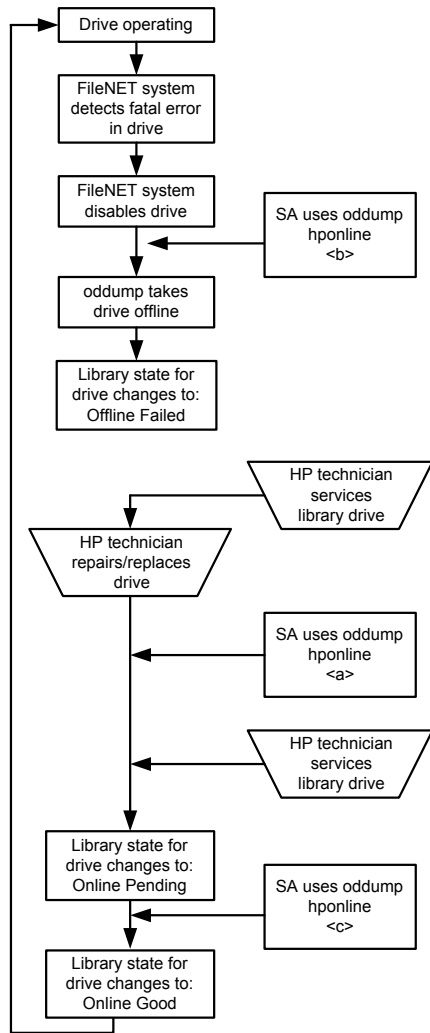
Drive State Diagram for Single-Drive Bracket Storage Library
